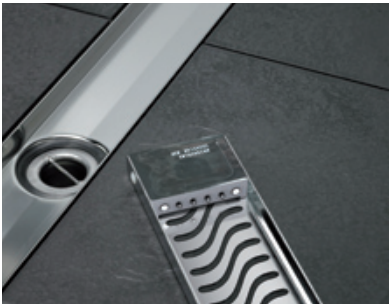
Insert LED modules and fix with the help of supplied plastic pins, then re-insert the grating
