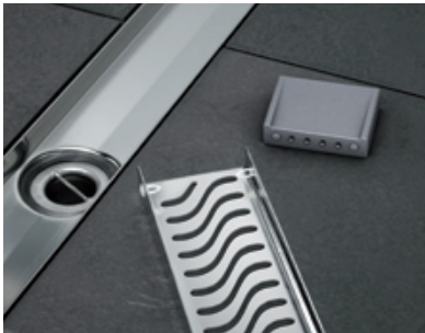
Remove the grating with the lifting aid
